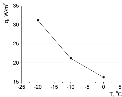
Figure 5. Heat flux test results of the element with reflective insulation for different values of outside temperature.
