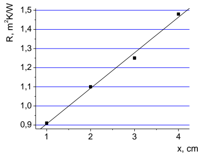
Figure 4. Dependency of thermal resistance as a function of the air gap width.
