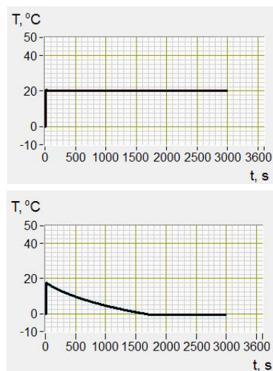
Figure 2. Temperature changes of the upper (heating) and lower (cooling) plates for sample with 2 cm air gap.
