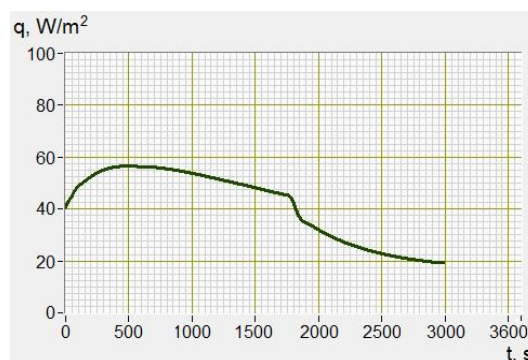
Figure 3. Changes of heat flux in time for sample with 2 cm air gap.
